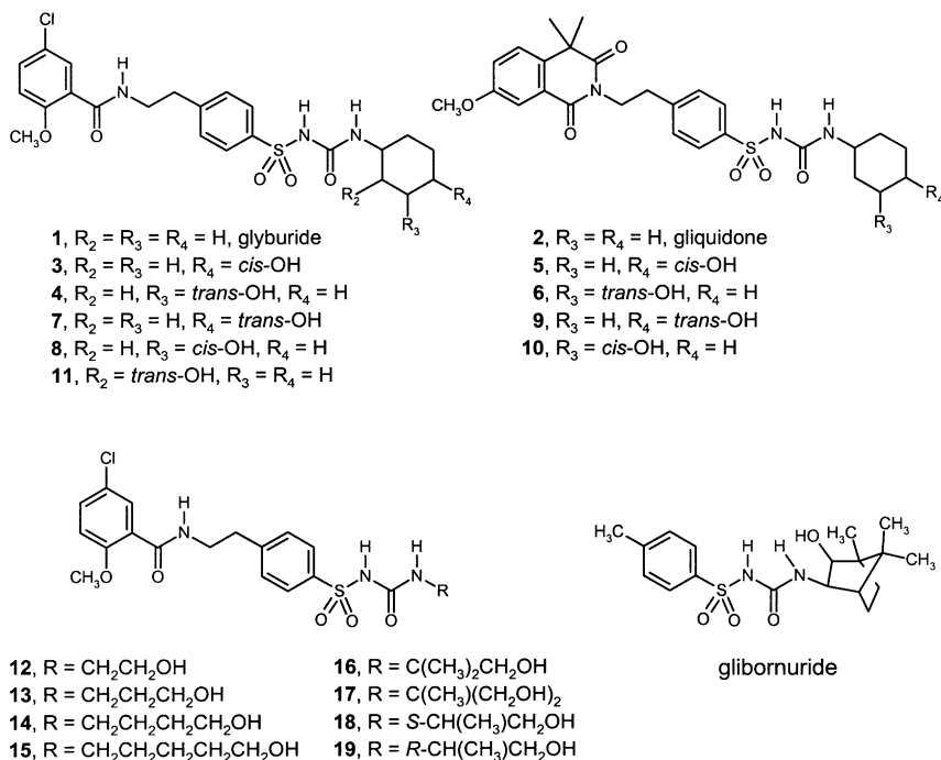
Scheme 1. Reagents: (a) phthalic anhydride, K_2CO_3 , DMAP, pyridine; (b) (i) K_2CO_3 , acetone; (ii) ClCO_2Et , reflux; (c) (i) cis/trans -4-aminocyclohexanol (2 equiv), dioxane, reflux; (ii) column chromatography; (d) (i) cis/trans -3-aminocyclohexanol (2 equiv), dioxane, reflux; (ii) column chromatography; (e) amino alcohol (2 equiv), dioxane, reflux.
