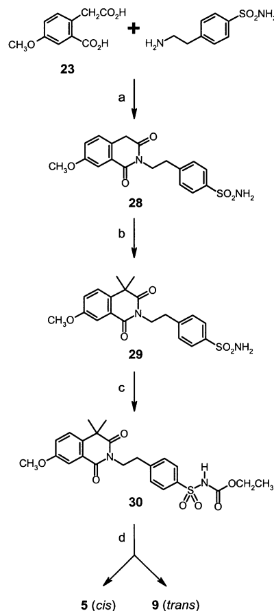
Scheme 3. Reagents: (a) melt, 200 °C; (b) 2 equiv NaOEt, 2 equiv CH 3 I, anhyd CH 3 OH; (c) (i) K 2 CO 3 , acetone; (ii) ClCO 2 Et, reflux; (d) (i) cis/trans -4-aminocyclohexanol, dioxane, reflux; (ii) column chromatography.
