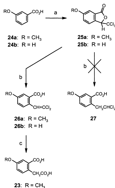
Scheme 2. Reagents: (a) Cl 3 CCH(OH) 2 , concd H 2 SO 4 , 24 h; (b) Zn°, CH 3 CO 2 H; (c) warm concd H 2 SO 4 .
