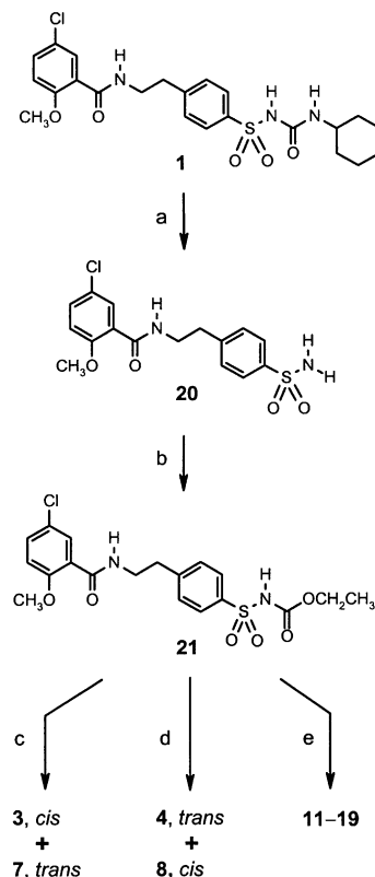
Scheme 1. Reagents: (a) phthalic anhydride, K_2CO_3 , DMAP, pyridine; (b) (i) K_2CO_3 , acetone; (ii) ClCO_2Et , reflux; (c) (i) cis/trans -4-aminocyclohexanol (2 equiv), dioxane, reflux; (ii) column chromatography; (d) (i) cis/trans -3-aminocyclohexanol (2 equiv), dioxane, reflux; (ii) column chromatography; (e) amino alcohol (2 equiv), dioxane, reflux.
