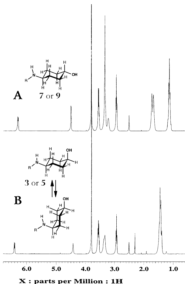
Figure 3. ^1\text{H} NMR of compounds 3 (A) and 7 (B), aliphatic regions.
